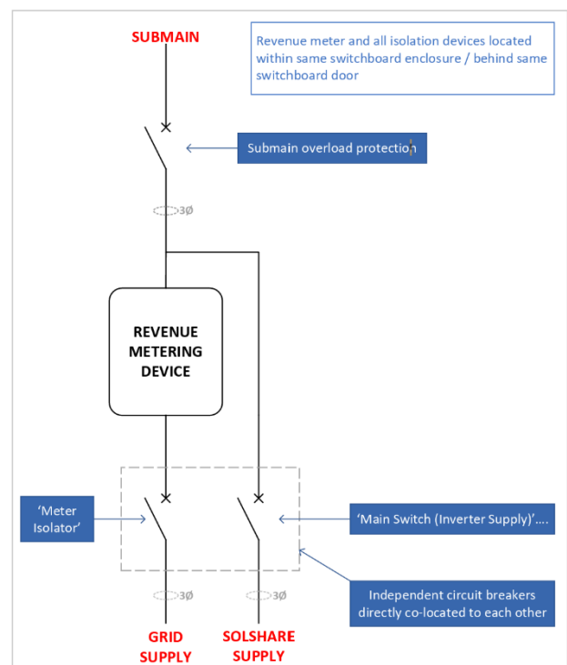
Preferred Wiring Arrangement for Three-Phase SolShare Connection
