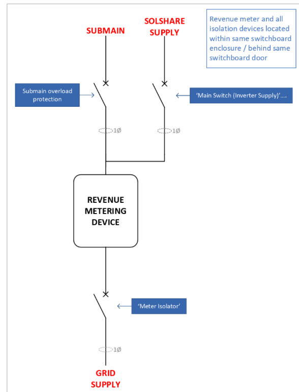
Alternative Wiring Arrangement for Single-Phase SolShare Connection
