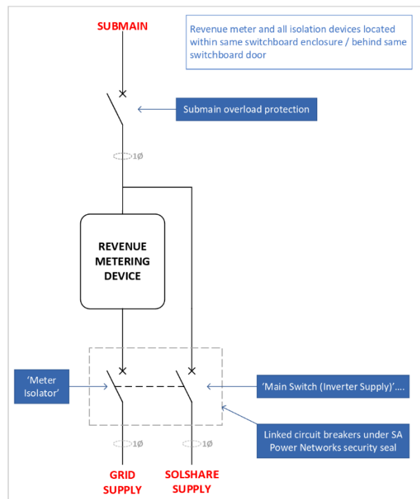
Preferred Wiring Arrangement for Single-Phase SolShare Connection
